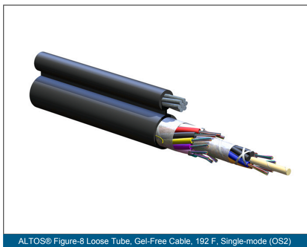
ALTOS® Figure-8 Loose Tube, Gel-Free Cable, 192 F, Single-mode (OS2)
