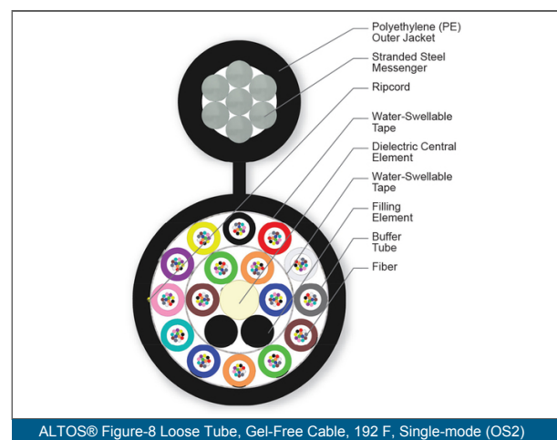
ALTOS® Figure-8 Loose Tube, Gel-Free Cable, 192 F, Single-mode (OS2)
